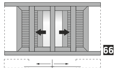
Double narrow sash pocket sliding window in 90° assembly in meeting stile with shutters Δίφυλλο χωνευτό με 90° κοπή, με παντζούρι
